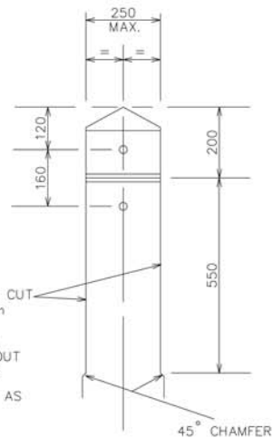
DETAIL A' SCALE 1:10
